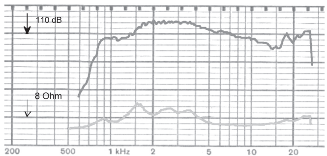
BMS 4540 ND, CD 90/75 Horn, SPL 1W / 1m
